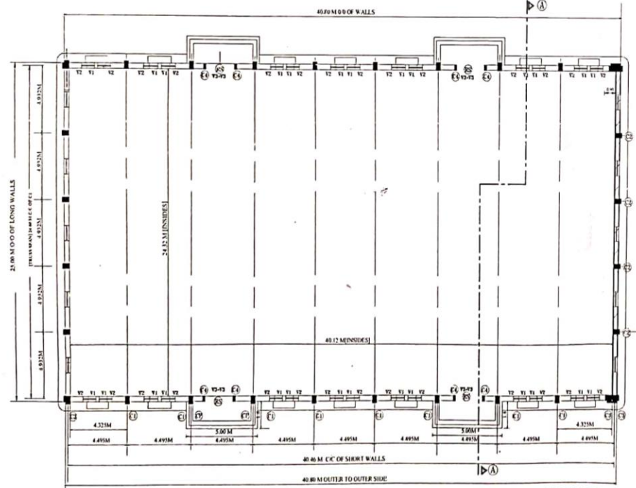
PLAN FOR 1800 MT. WAREHOUSE UNIT NO. I, II
